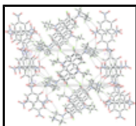
Fig. 2. The crystal packing of the title compound, showing hydrogen-bonded (dashed lines) network.
